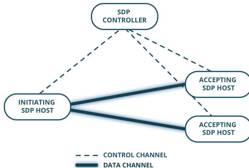
Figure 1: Software Defined Perimeter Architecture
